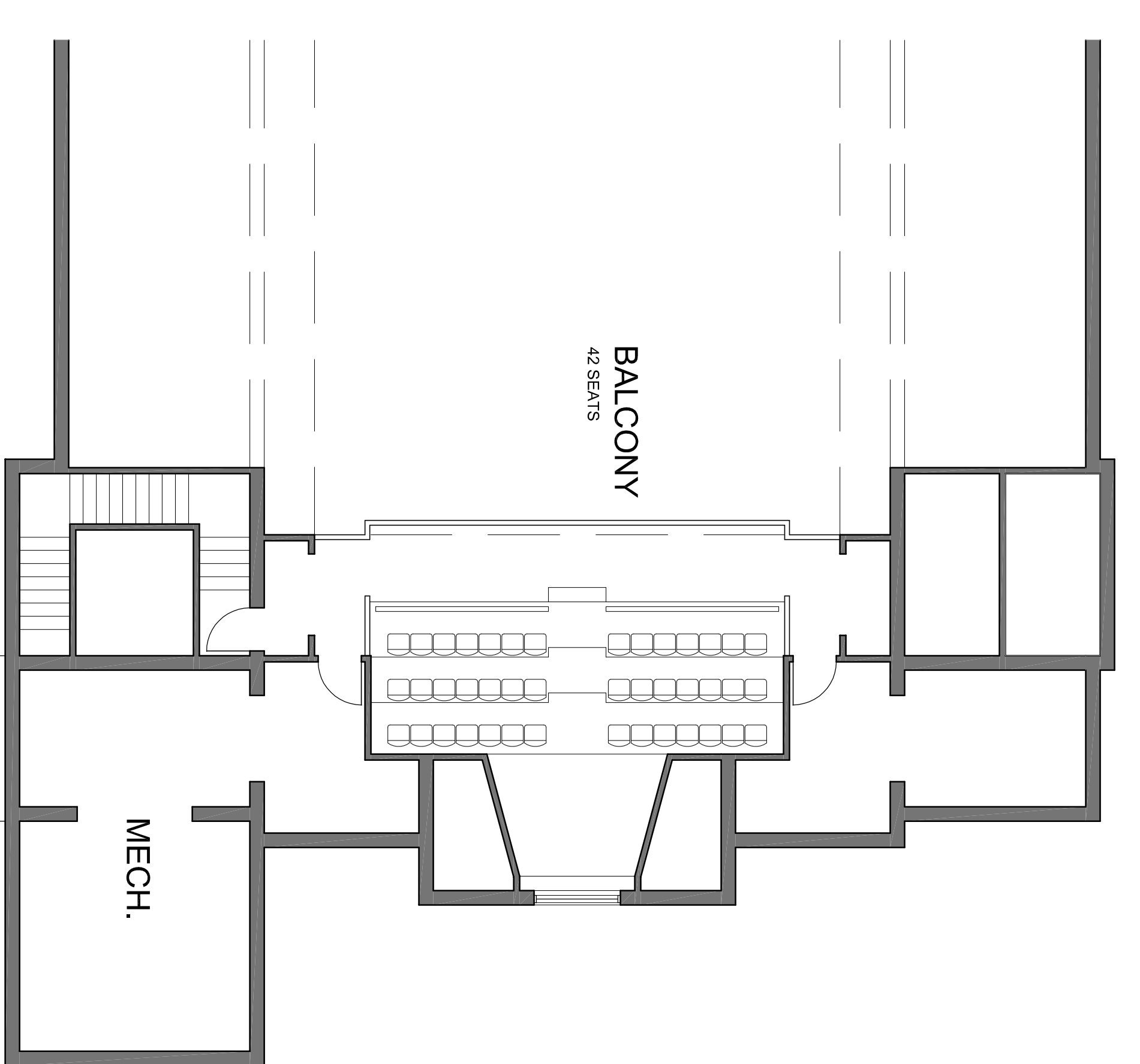
Balcony Plan
